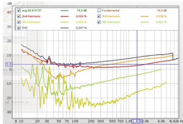
U101, vasak kanal, 24,5W@5,4Ω.
