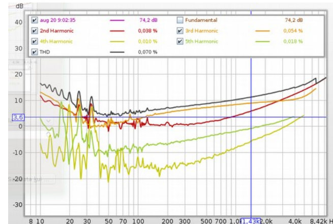
U101, parem kanal, 24,5W@5,4Ω.
